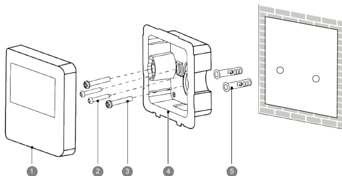
Parts of Wired Controller
